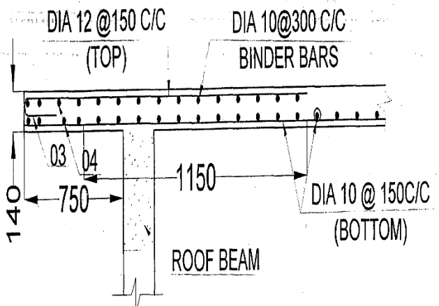
SECTION K-K
