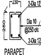
PARAPET BEAM
