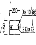
SILL BEAM
