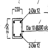
LINTEL BEAM -1
