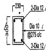
PLINTH BEAM
