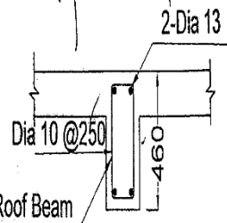
ROOF BEAM
